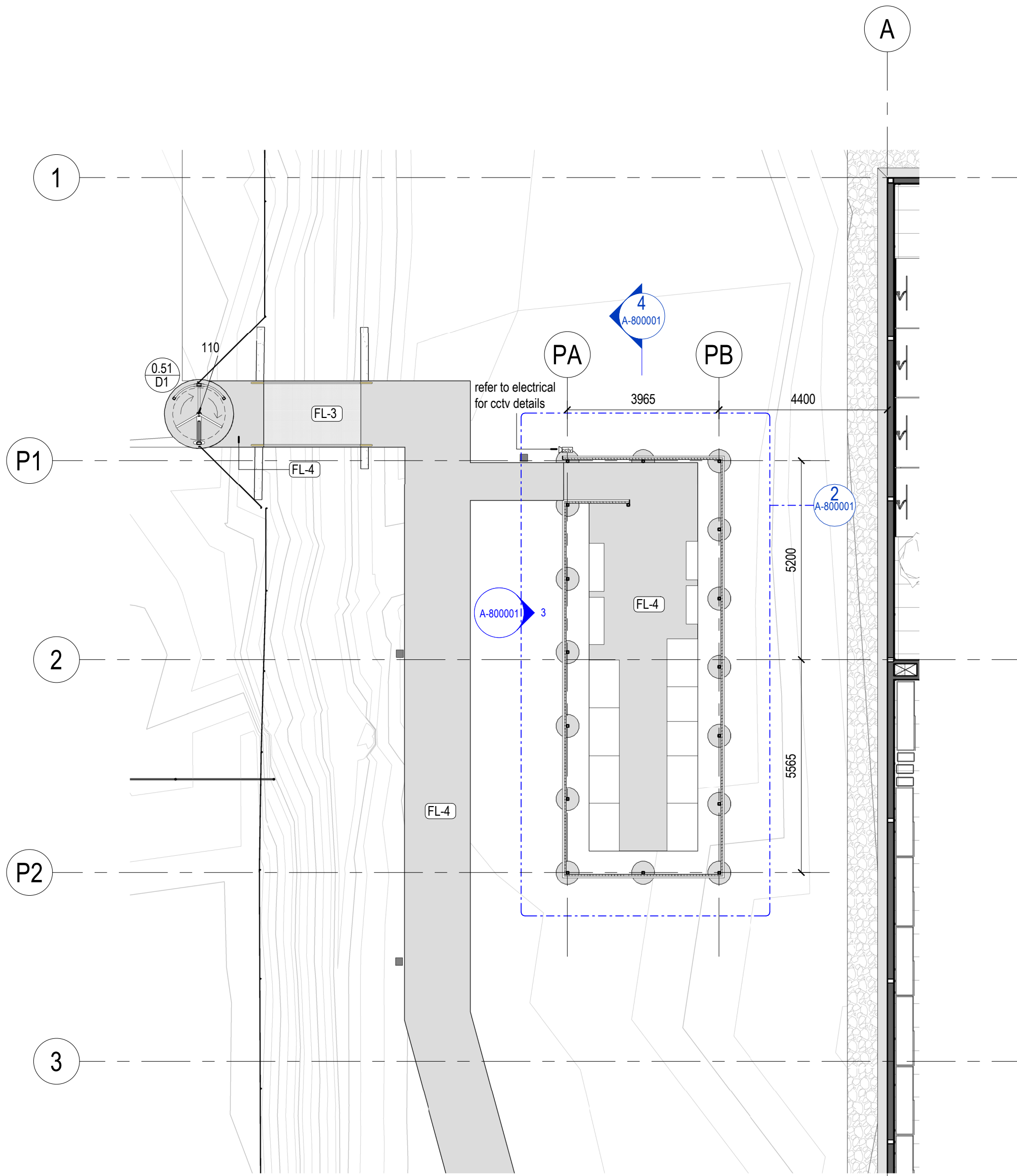
1 Plant Room Site Plan 1 : 100
