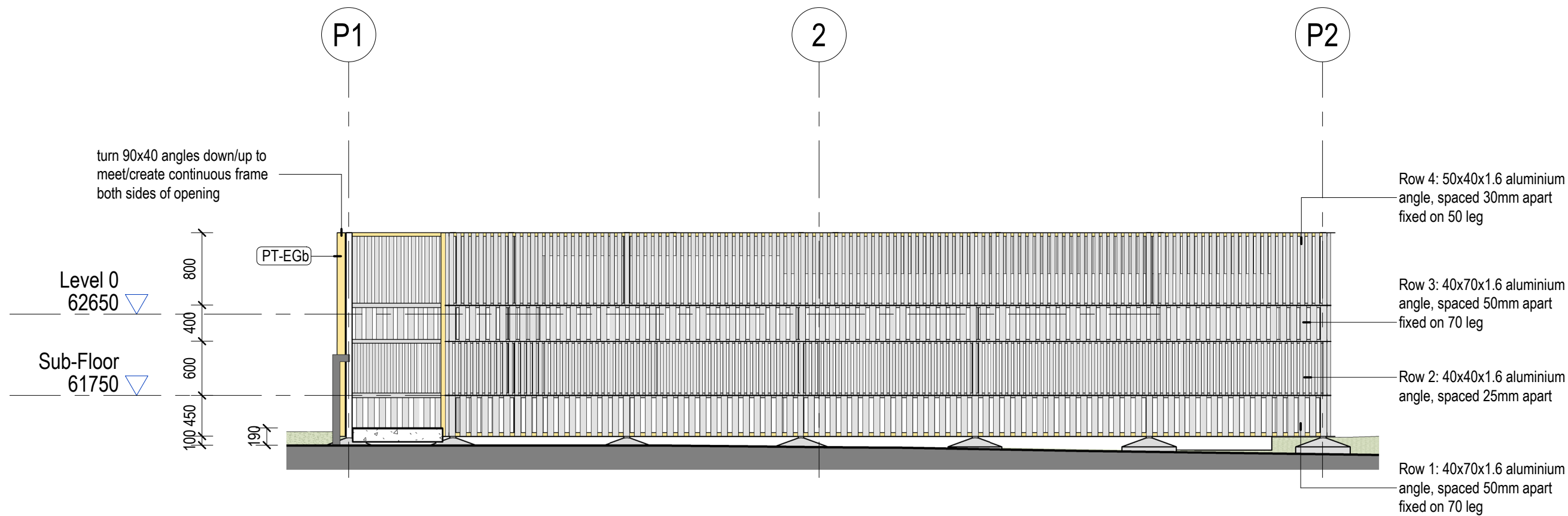
3 80 N Plant Room Elevation 1 : 50
