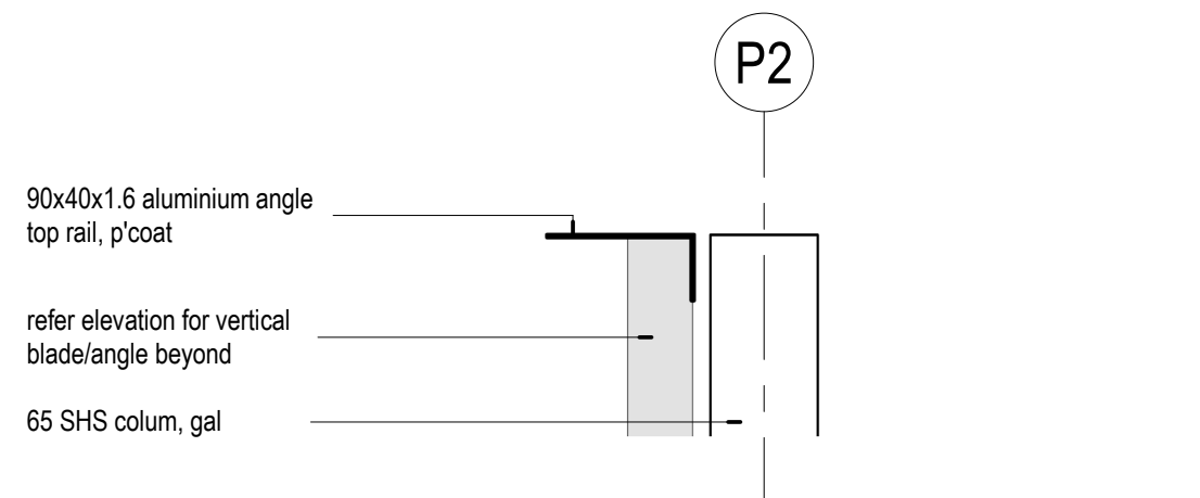
5 Plant Room Detail Section A 1 : 5
