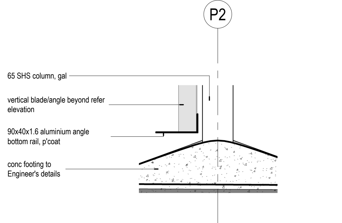
7 Plant Room Detail Section C 1 : 5
