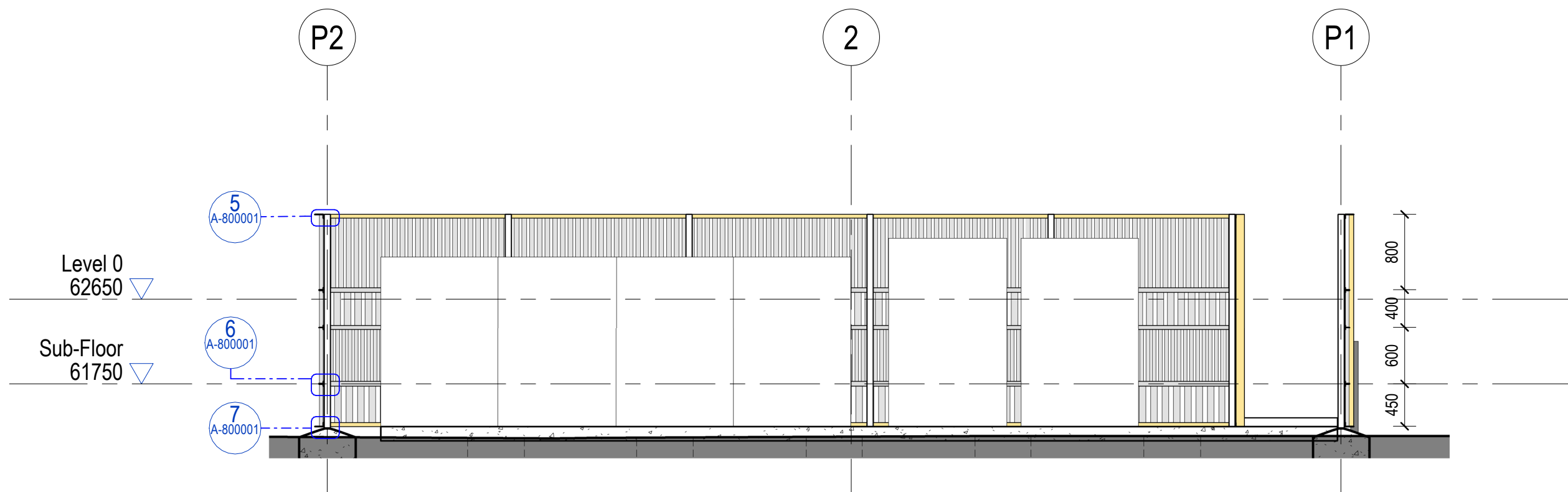
4 Plant Room Section 1 : 50
