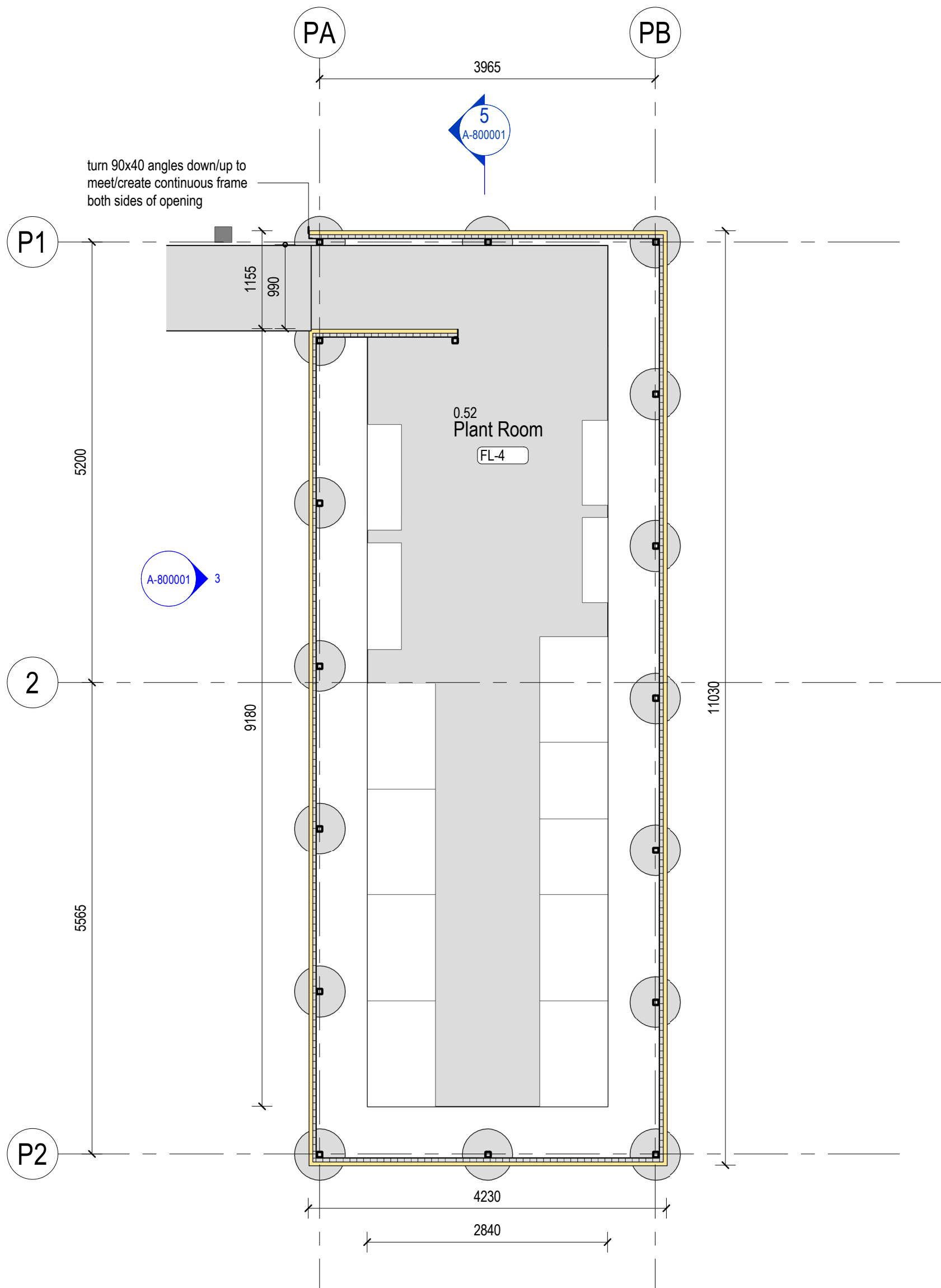
2 Plant Room Floor Plan 1 : 50
