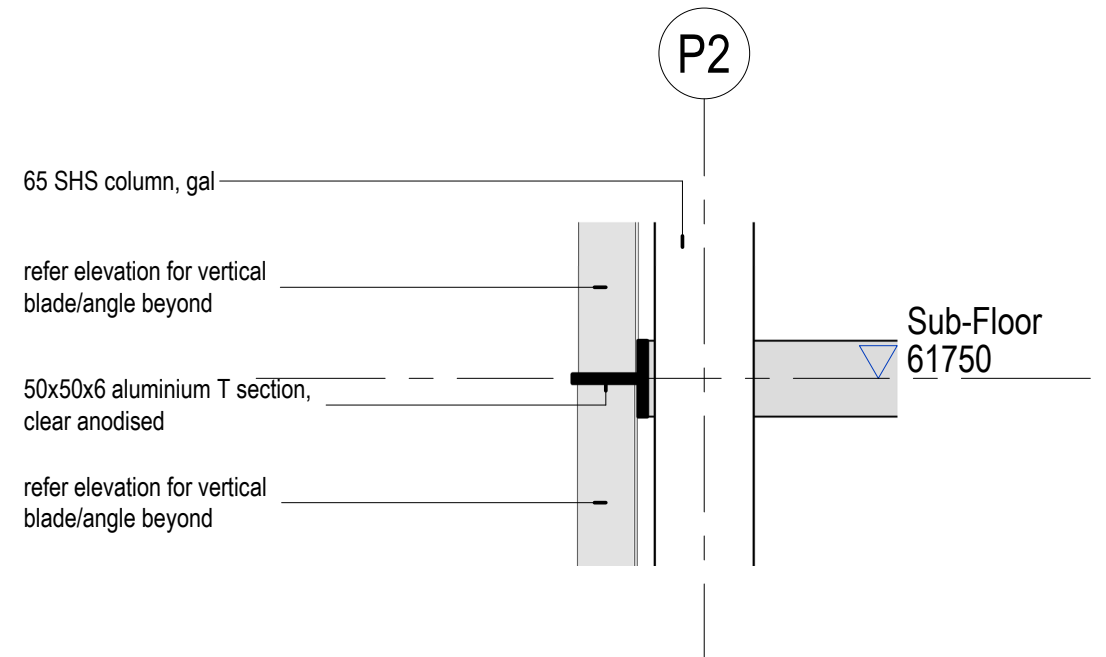
6 Plant Room Detail Section B 1 : 5
